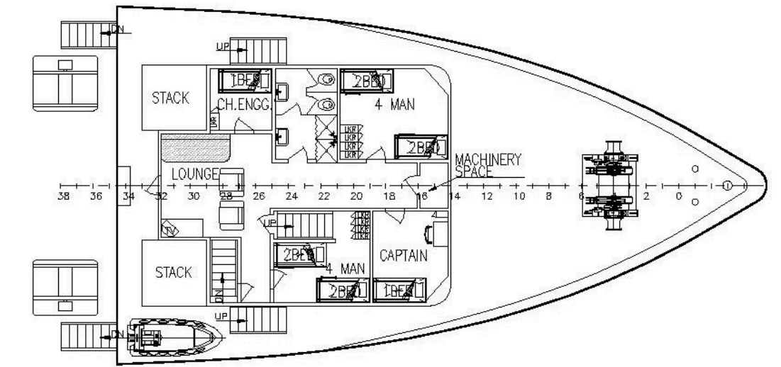
FORECASTLE DECK PLAN
