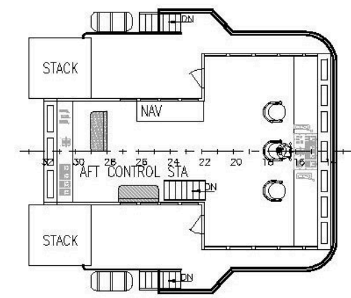
BRIDGE DECK
