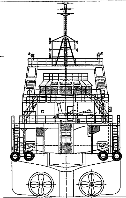
STERN VIEW
